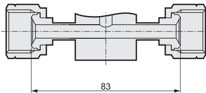
암피팅: 6R
