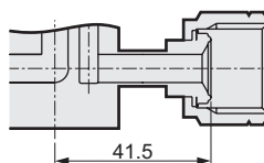
암피팅: 6R
